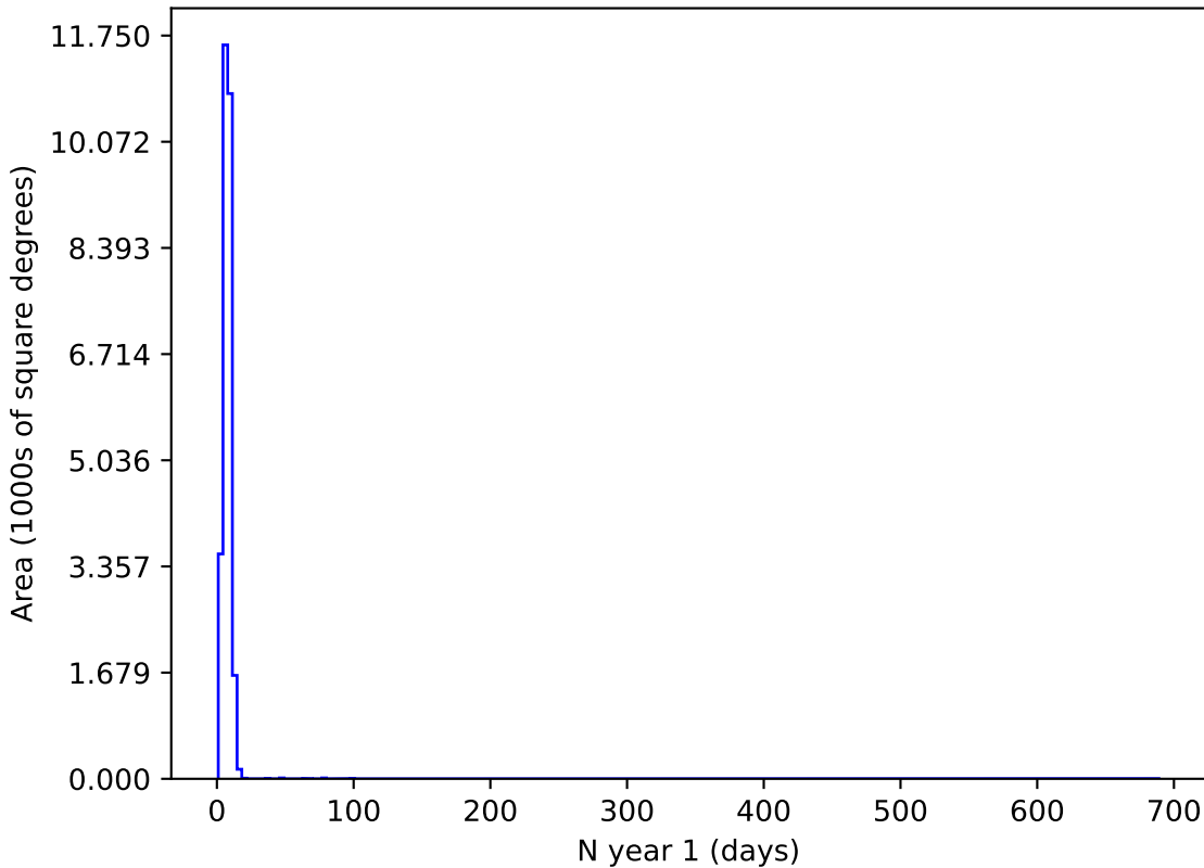
ddf_loaded_fl4_v3.4_10yrs g and night &lt; 365: N year 1
