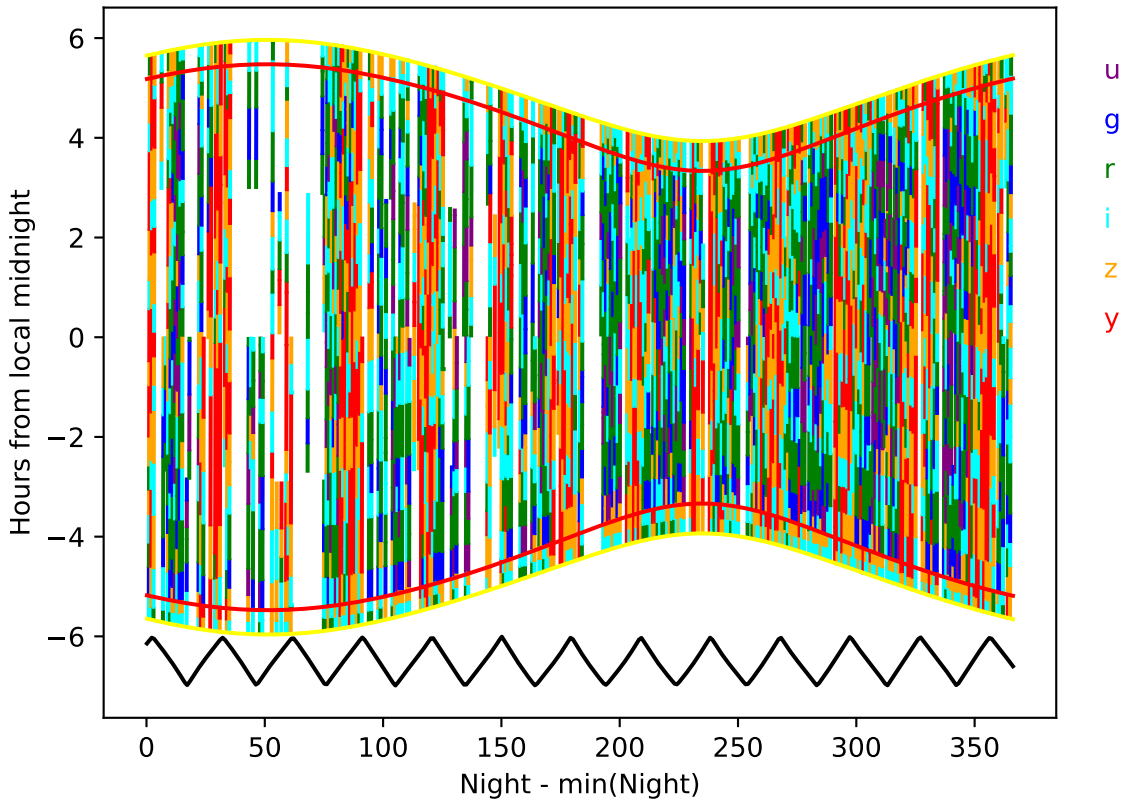
ddf_loaded_fl4_v3.4_10yrs year 9-10: Hourglass
