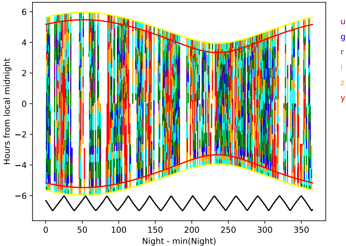
ddf_loaded_fl4_v3.4_10yrs year 7-8: Hourglass
