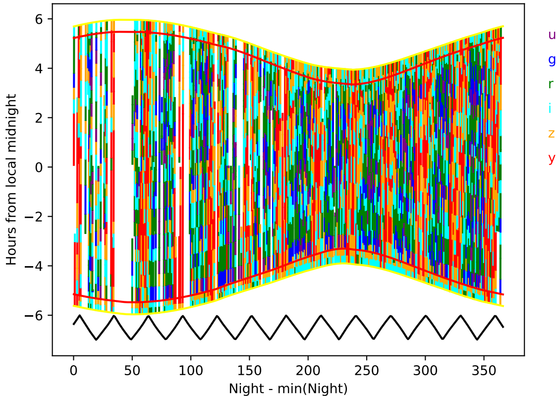
ddf_loaded_fl4_v3.4_10yrs year 6-7: Hourglass
