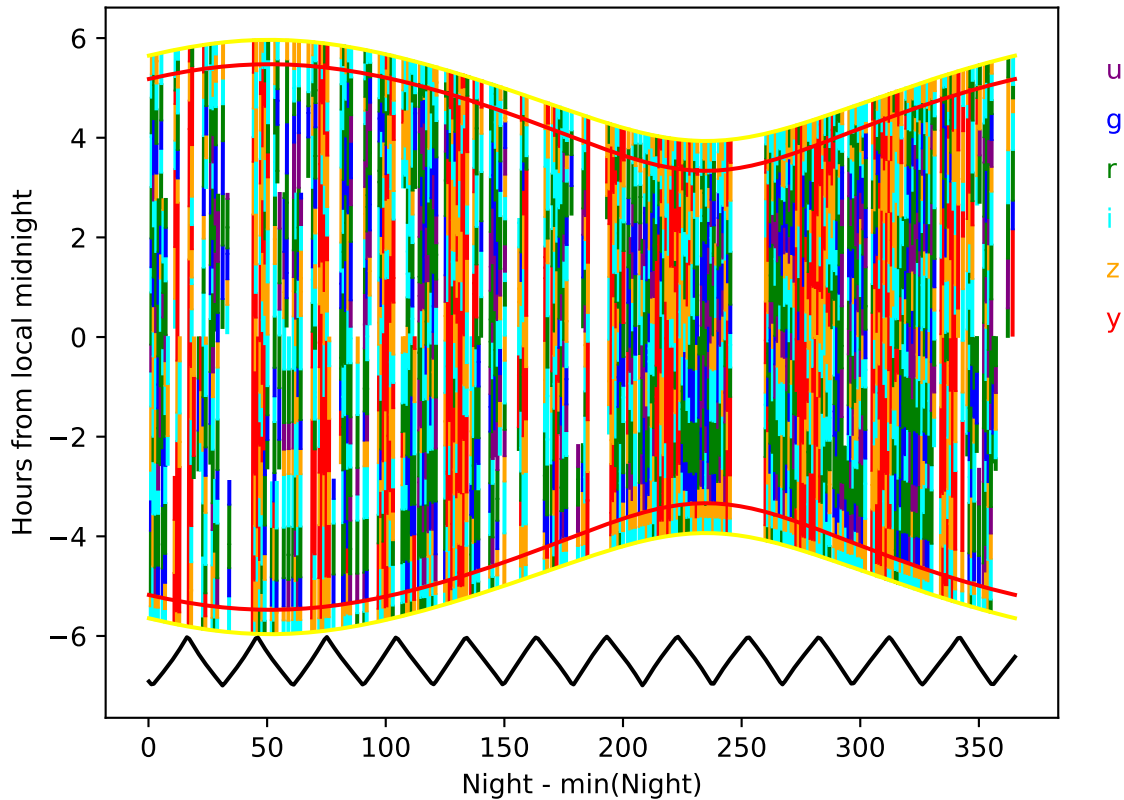
ddf_loaded_fl4_v3.4_10yrs year 5-6: Hourglass
