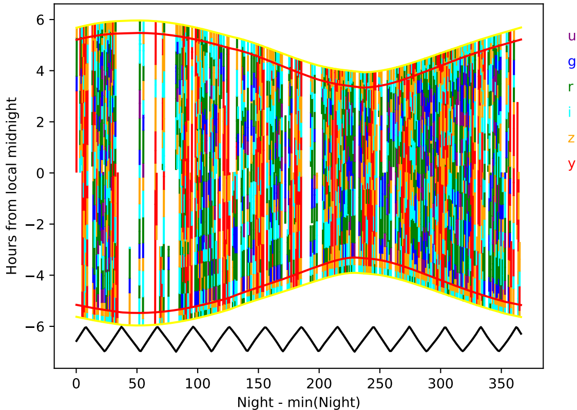
ddf_loaded_fl4_v3.4_10yrs year 3-4: Hourglass
