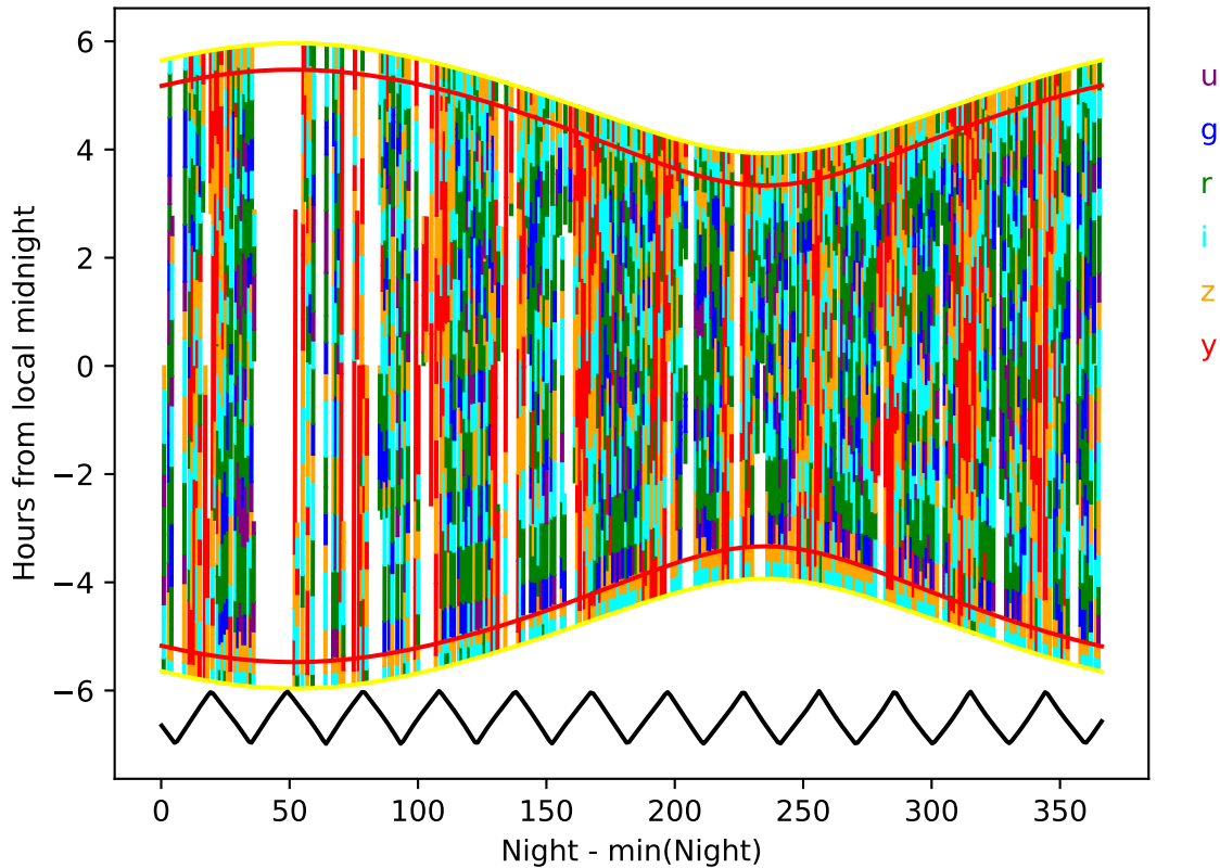
ddf_loaded_fl4_v3.4_10yrs year 2-3: Hourglass
