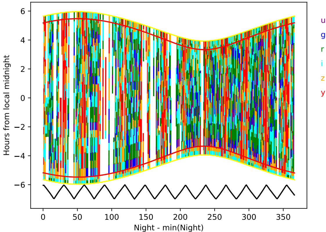
ddf_loaded_fl4_v3.4_10yrs year 1-2: Hourglass
