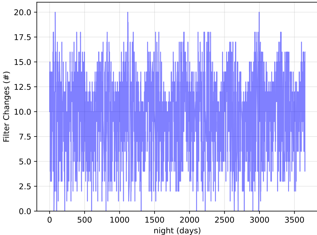
ddf_loaded_fl4_v3.4_10yrs : Filter Changes
