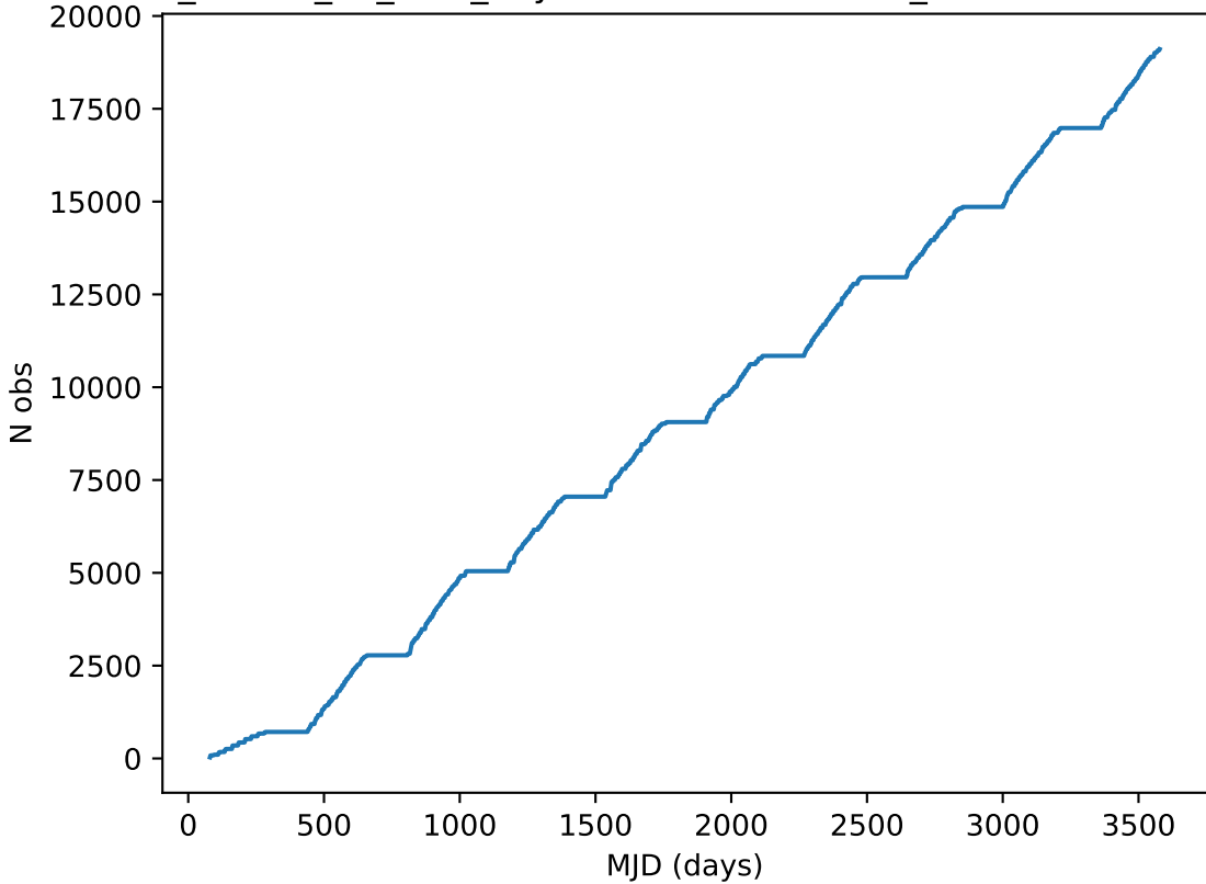
ddf_loaded_fl4_v3.4_10yrs note like DD:XMM_LSS%: Cumulative
