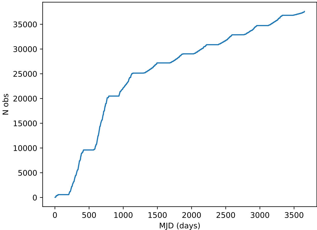
ddf_loaded_fl4_v3.4_10yrs note like DD:COSMOS%: Cumulative
