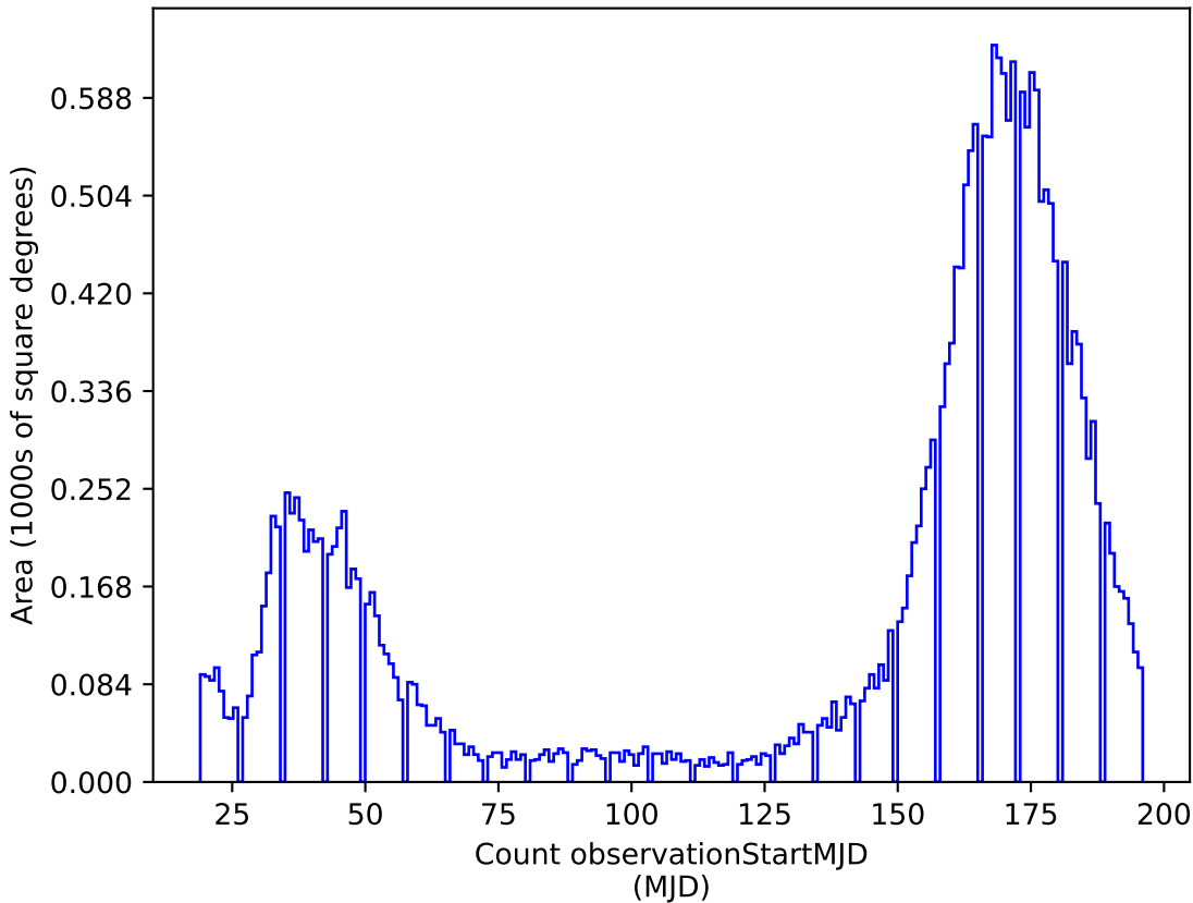
ddf_loaded_fl4_v3.4_10yrs z: Count observationStartMJD
