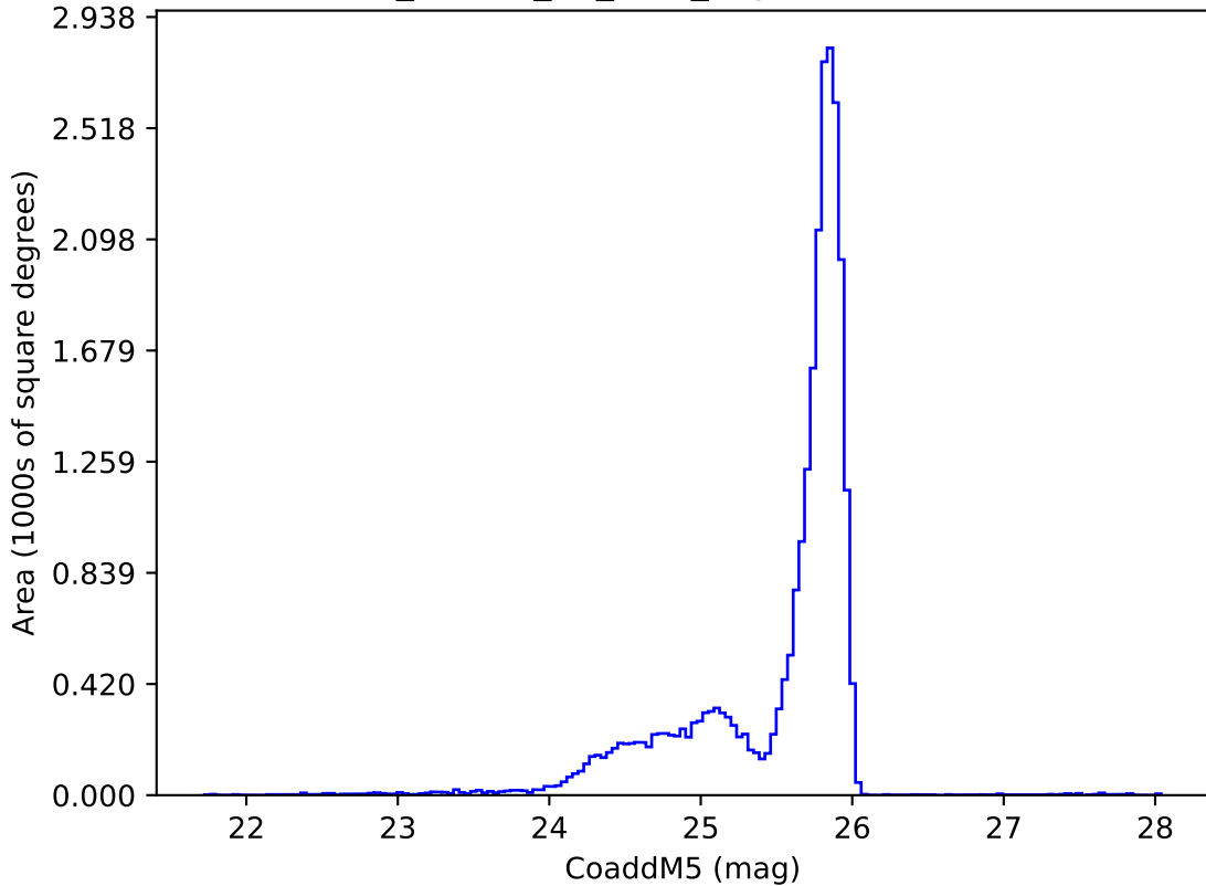
ddf_loaded_fl4_v3.4_10yrs z: CoaddM5
