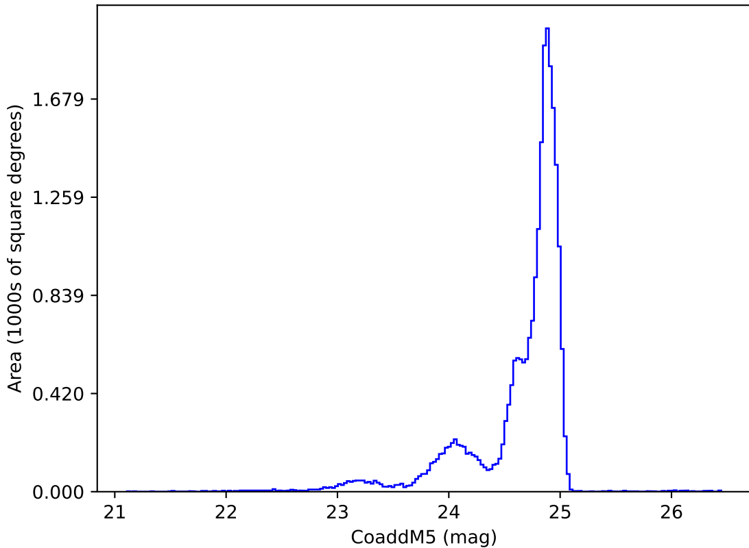
ddf_loaded_fl4_v3.4_10yrs y: CoaddM5
