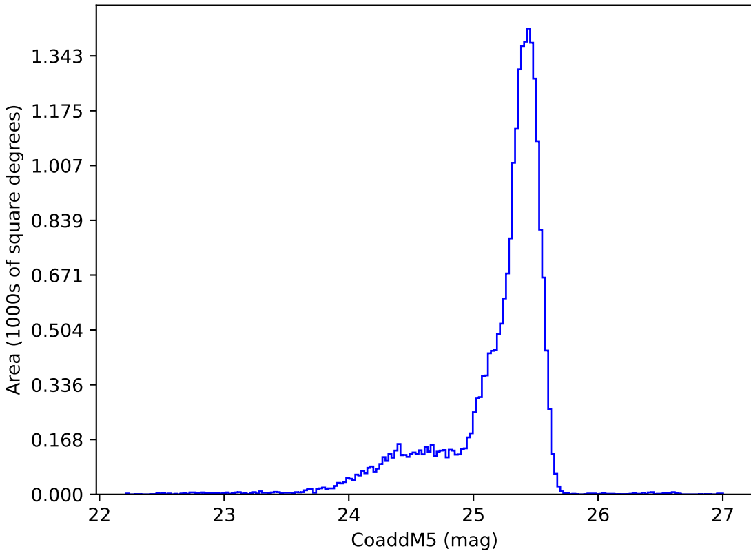
ddf_loaded_fl4_v3.4_10yrs u: CoaddM5
