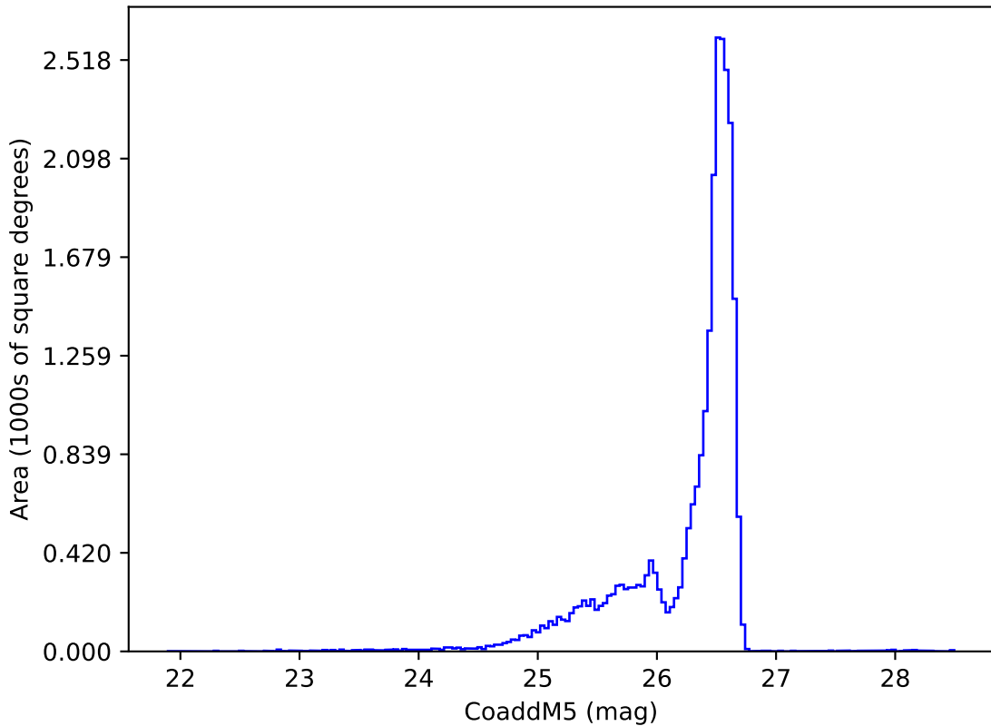
ddf_loaded_fl4_v3.4_10yrs i: CoaddM5
