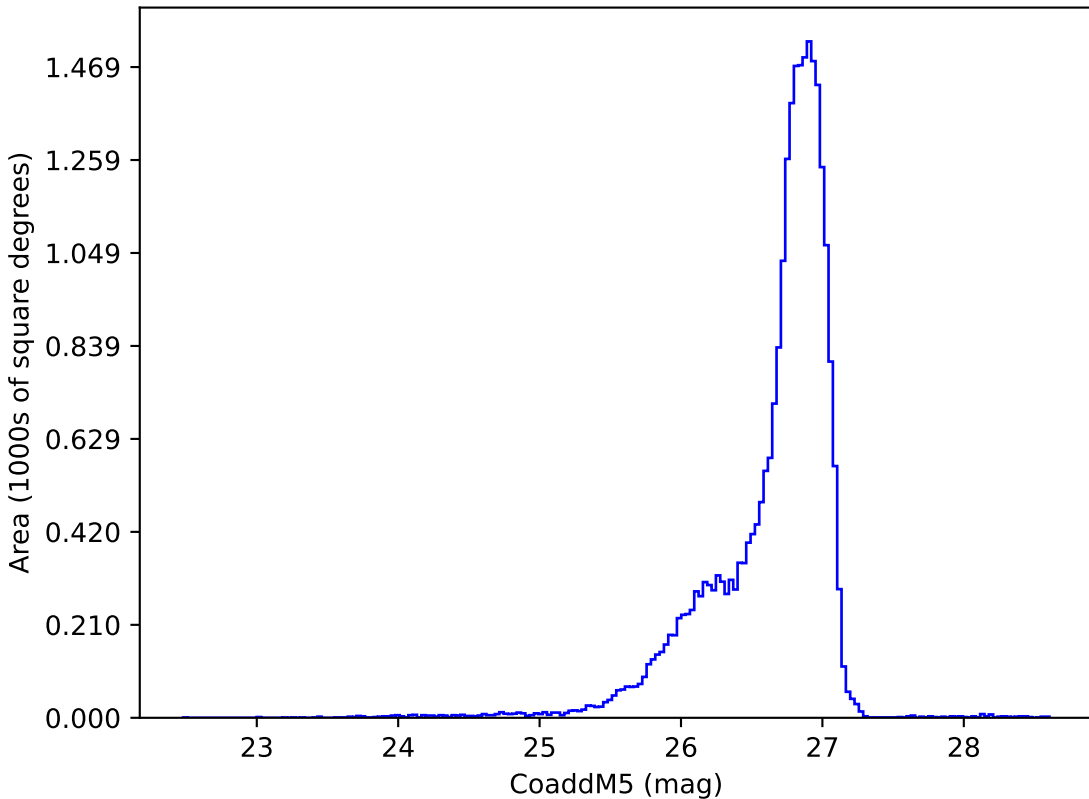
ddf_loaded_fl4_v3.4_10yrs g: CoaddM5
