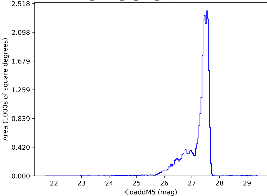
ddf_loaded_fl4_v3.4_10yrs : CoaddM5
