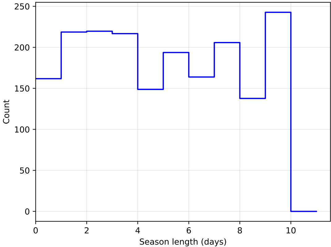
ddf_loaded_fl4_v3.4_10yrs DD:WFD all bands: SeasonLength
