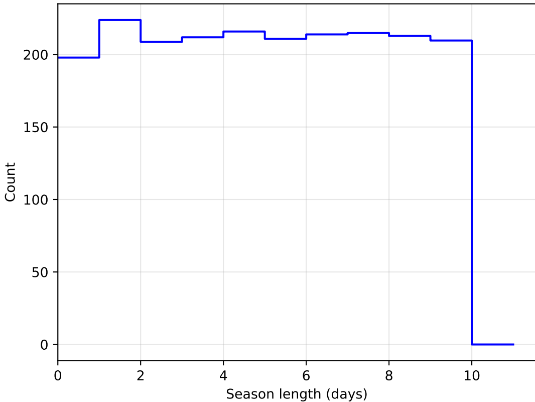
ddf_loaded_fl4_v3.4_10yrs DD:ELAISS1 all bands: SeasonLength
