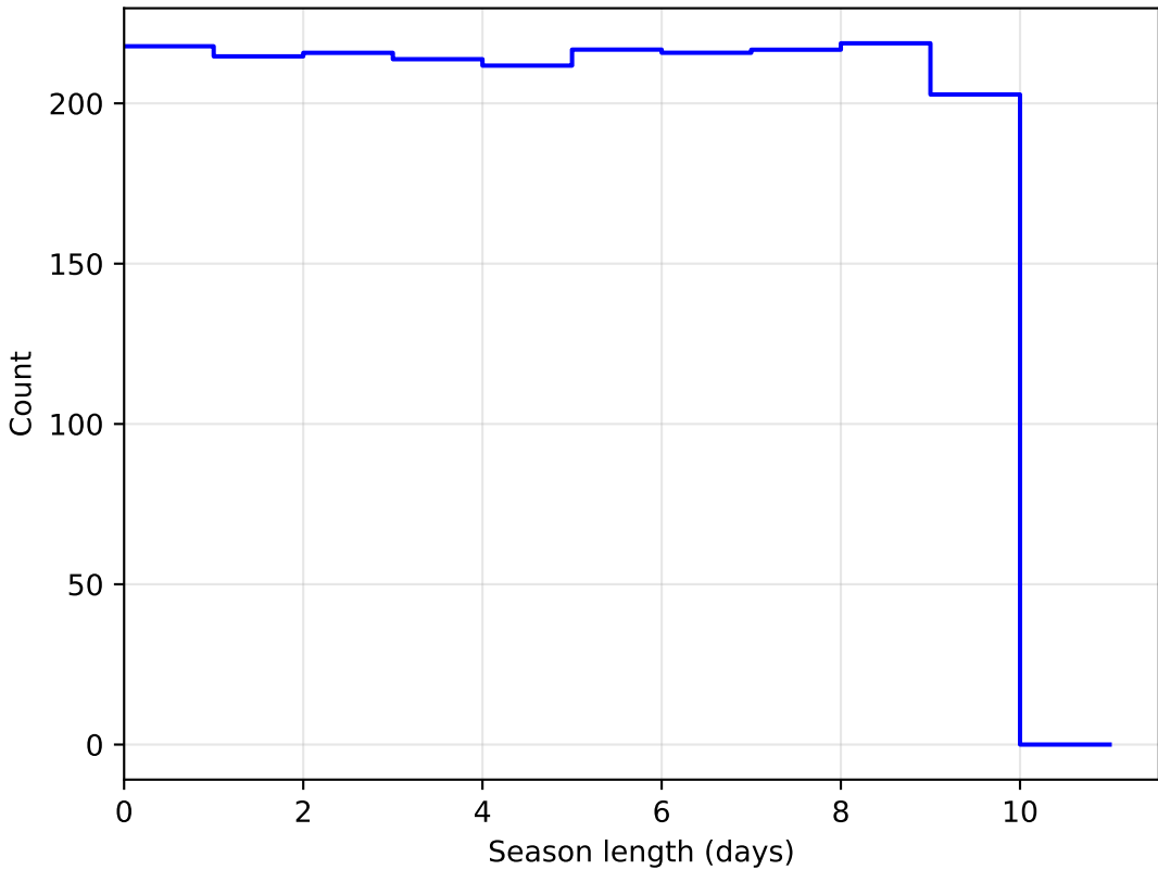
ddf_loaded_fl4_v3.4_10yrs DD:ECDFS all bands: SeasonLength
