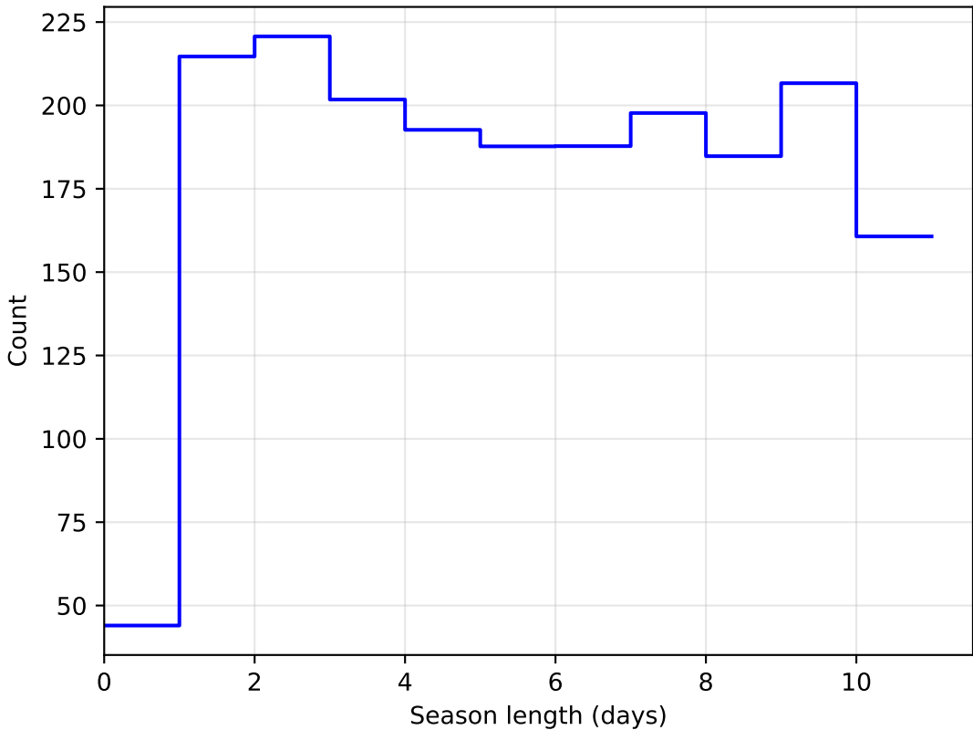
ddf_loaded_fl4_v3.4_10yrs DD: COSMOS all bands: SeasonLength
