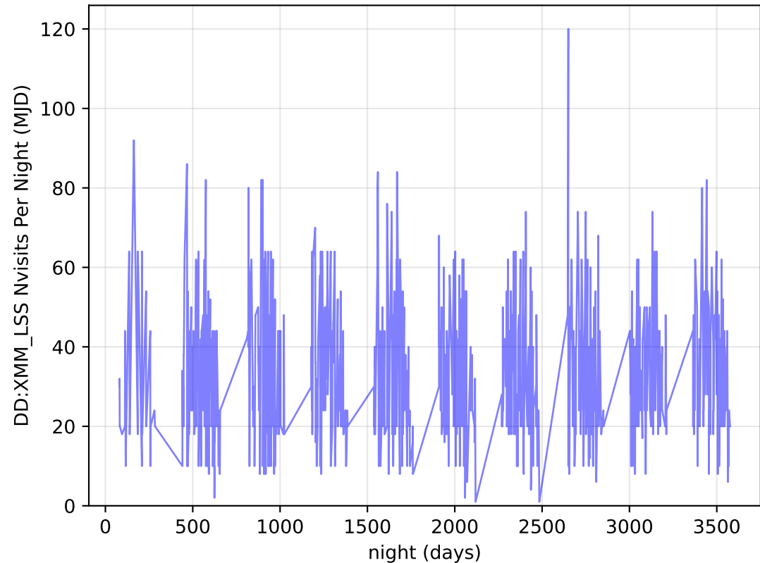
ddf_loaded_fl4_v3.4_10yrs all bands: DD:XMM_LSS Nvisits Per Night
