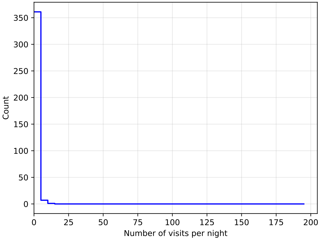
ddf_loaded_fl4_v3.4_10yrs all bands: DD:WFD NVisitsPerNight
