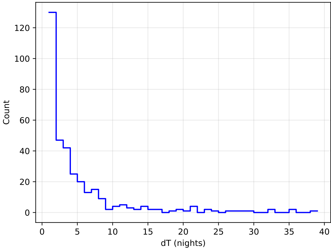
ddf_loaded_fl4_v3.4_10yrs all bands: DD:WFD Delta Nights Histogram
