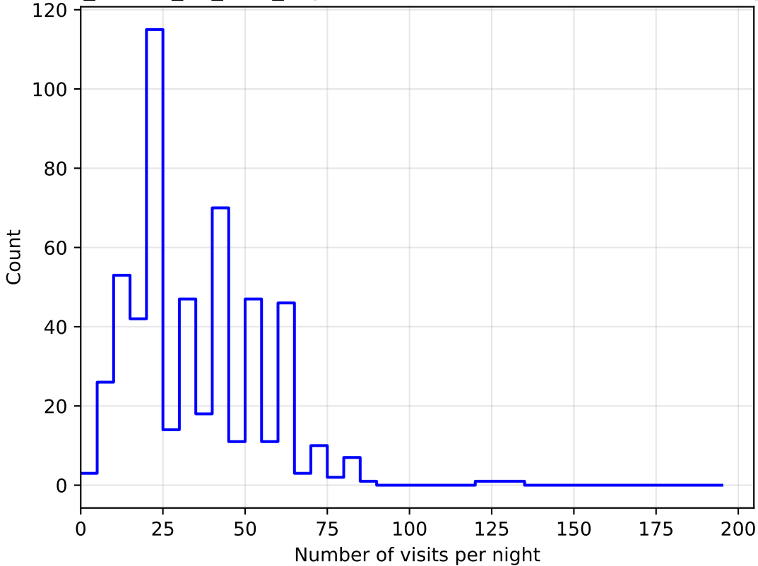
ddf_loaded_fl4_v3.4_10yrs all bands: DD:ELAISS1 NVisitsPerNight
