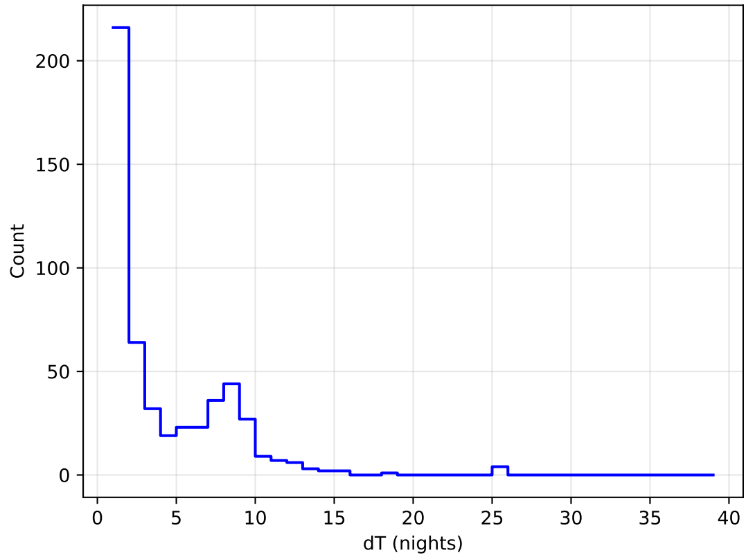
ddf_loaded_fl4_v3.4_10yrs all bands: DD:ELAISS1 Delta Nights Histogram
