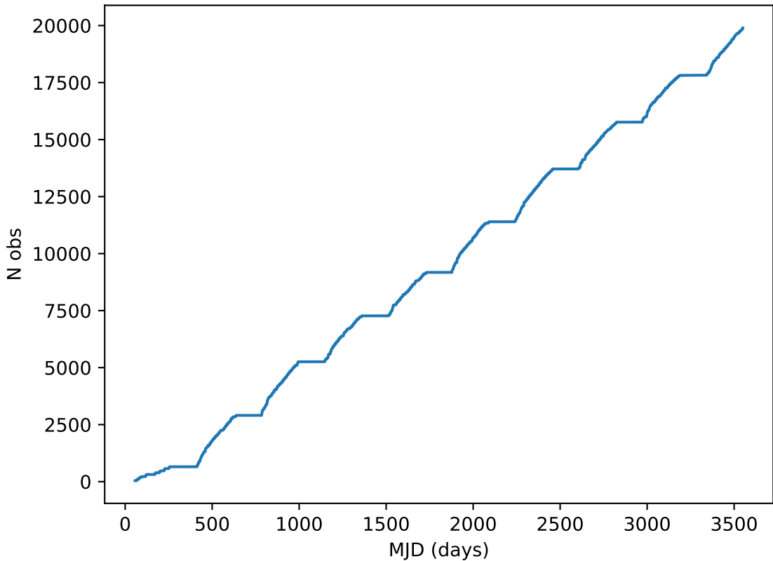
ddf_loaded_fl4_v3.4_10yrs all bands: DD:ELAISS1 Cumulative NVisits
