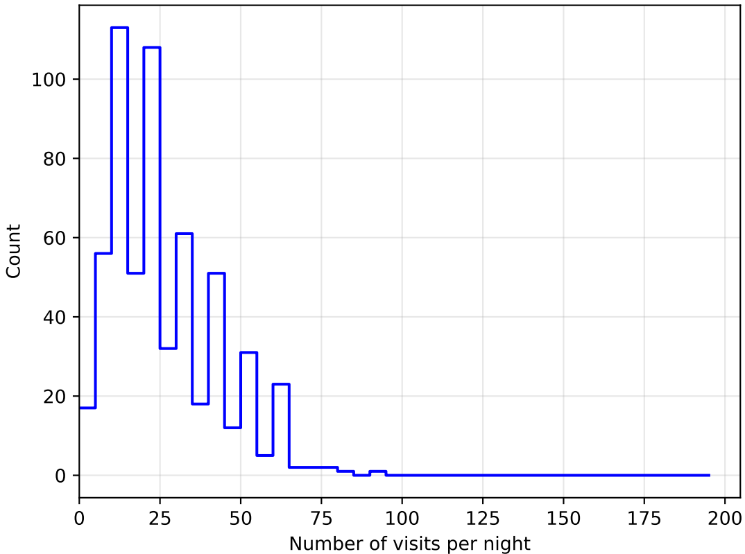
ddf_loaded_fl4_v3.4_10yrs all bands: DD:EDFS NVisitsPerNight
