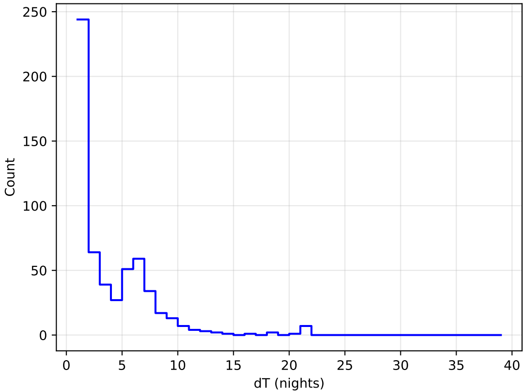
ddf_loaded_fl4_v3.4_10yrs all bands: DD:EDFS Delta Nights Histogram
