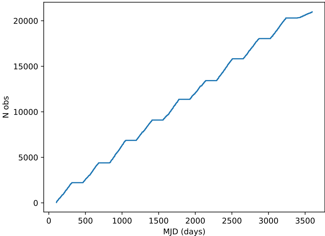
ddf_loaded_fl4_v3.4_10yrs all bands: DD:EDFS Cumulative NVisits
