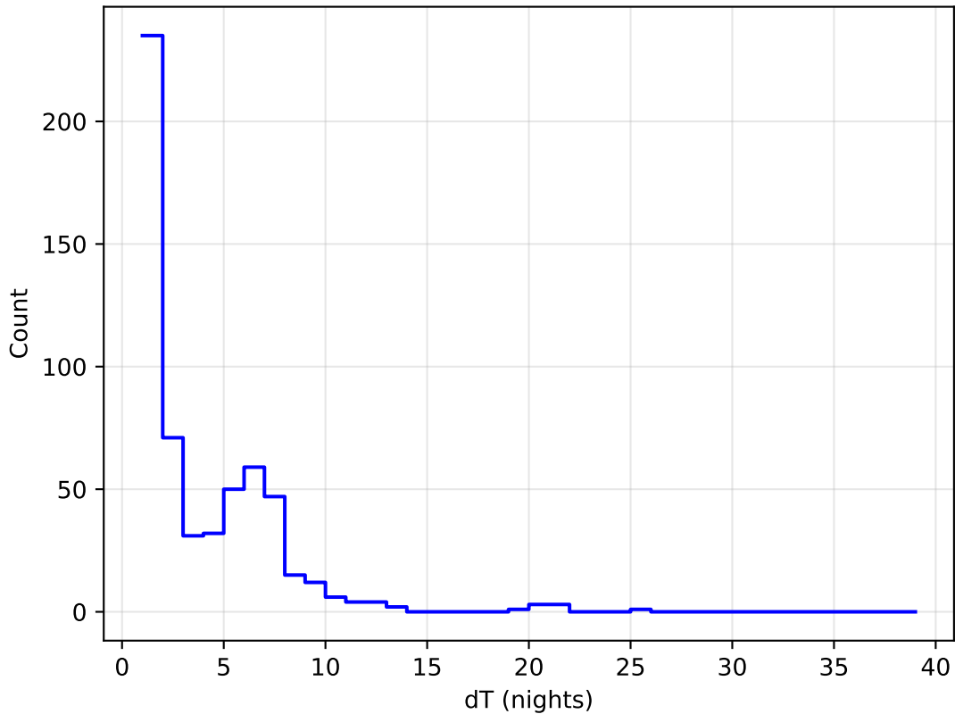
ddf_loaded_fl4_v3.4_10yrs all bands: DD:ECDFS Delta Nights Histogram
