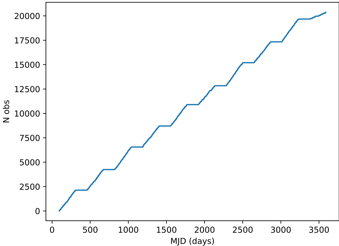
ddf_loaded_fl4_v3.4_10yrs all bands: DD:ECDFS Cumulative NVisits
