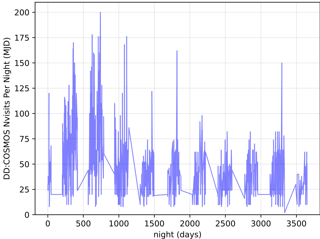
ddf_loaded_fl4_v3.4_10yrs all bands: DD:COSMOS Nvisits Per Night
