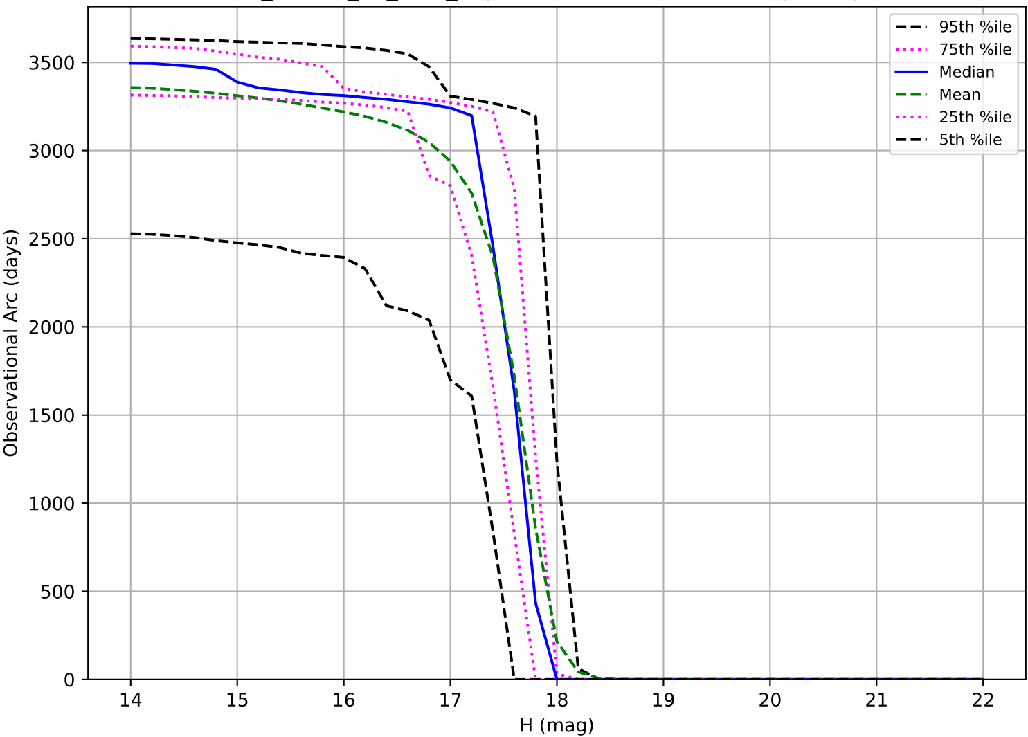
ddf_loaded_fl2_v3.4_10yrs: Observational Arc Length Trojan
