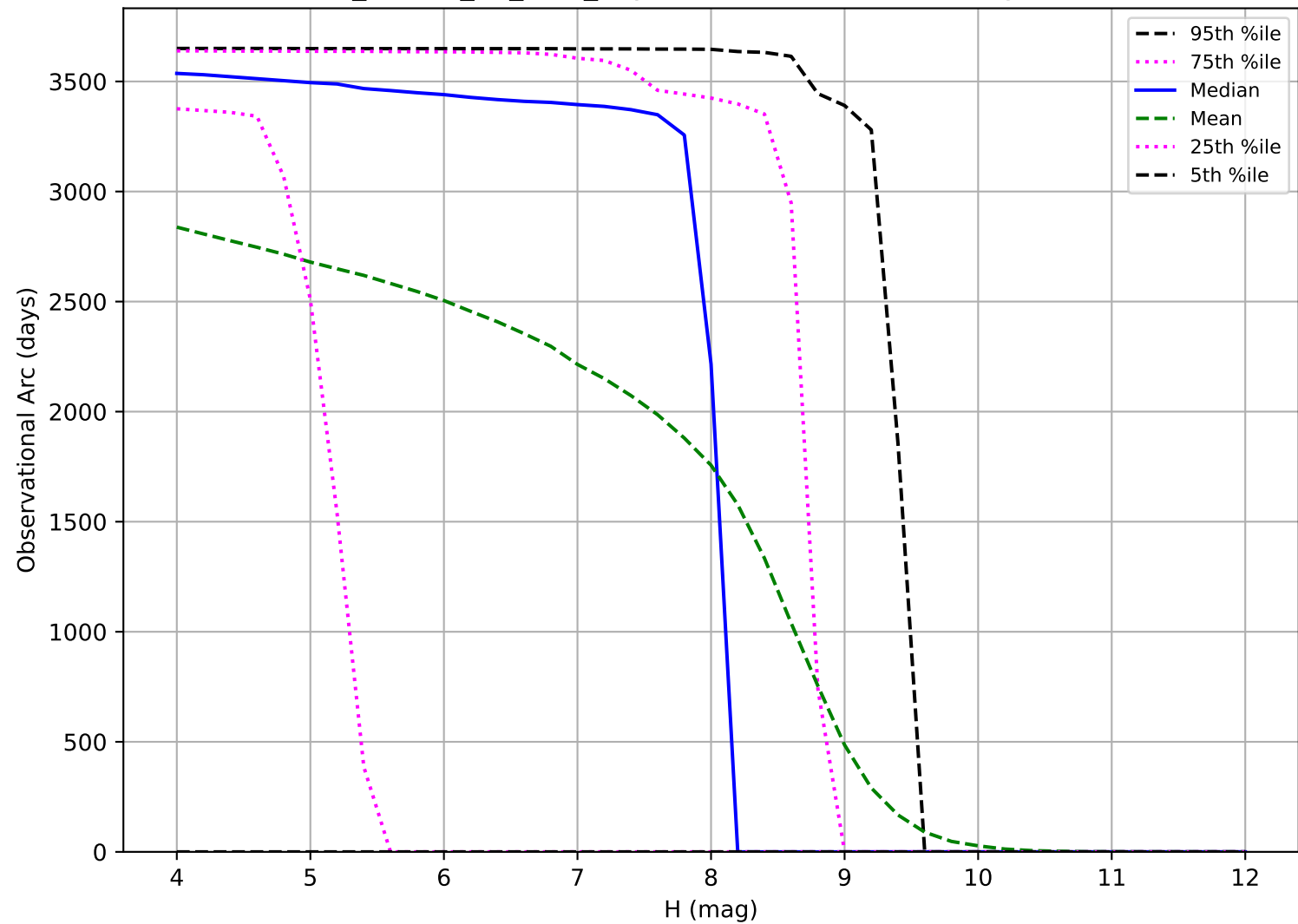
ddf_loaded_fl2_v3.4_10yrs: Observational Arc Length TNO
