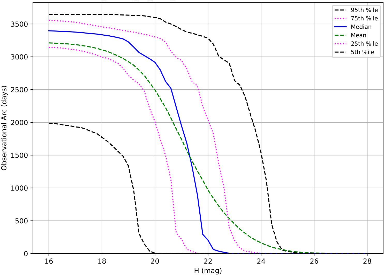
ddf_loaded_fl2_v3.4_10yrs: Observational Arc Length PHA
