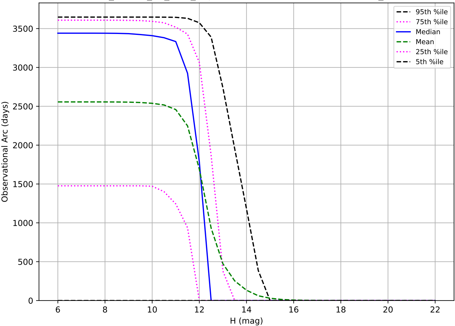
ddf_loaded_fl2_v3.4_10yrs: Observational Arc Length OCC_r20
