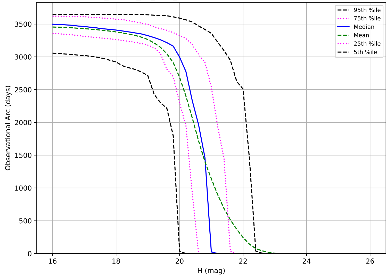
ddf_loaded_fl2_v3.4_10yrs: Observational Arc Length MBA
