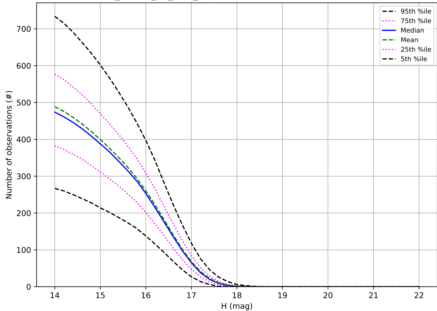
ddf_loaded_fl2_v3.4_10yrs: Number of observations Trojan
