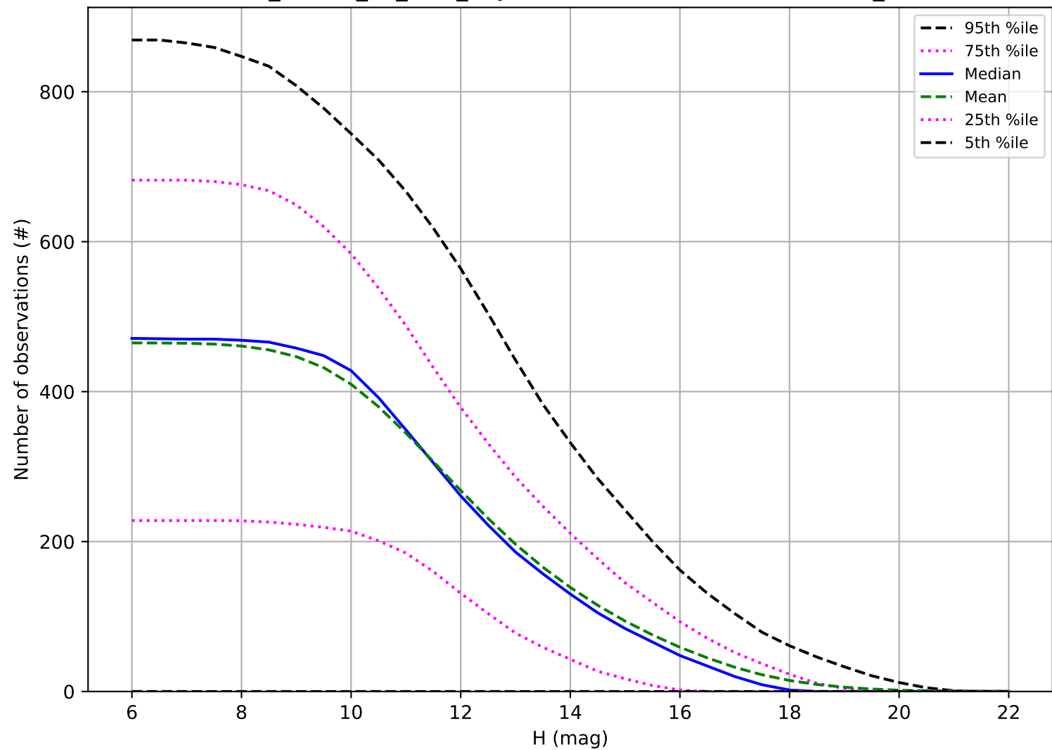
ddf_loaded_fl2_v3.4_10yrs: Number of observations OCC_r5
