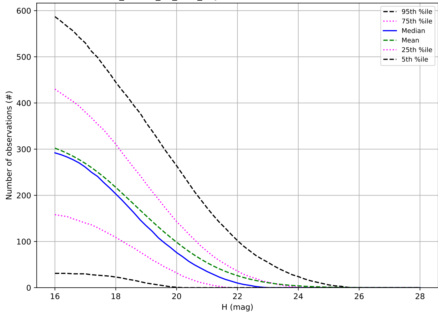
ddf_loaded_fl2_v3.4_10yrs: Number of observations NEO
