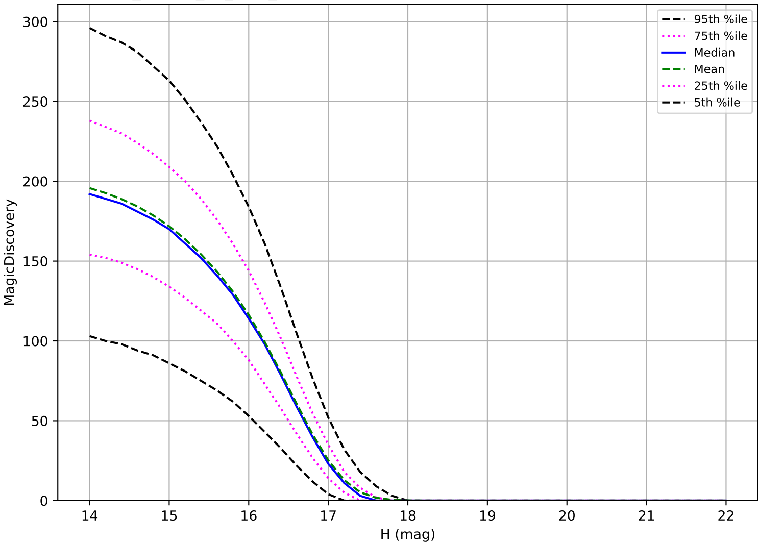
ddf_loaded_fl2_v3.4_10yrs: Trojan 6 detections in 60 nights detection loss
