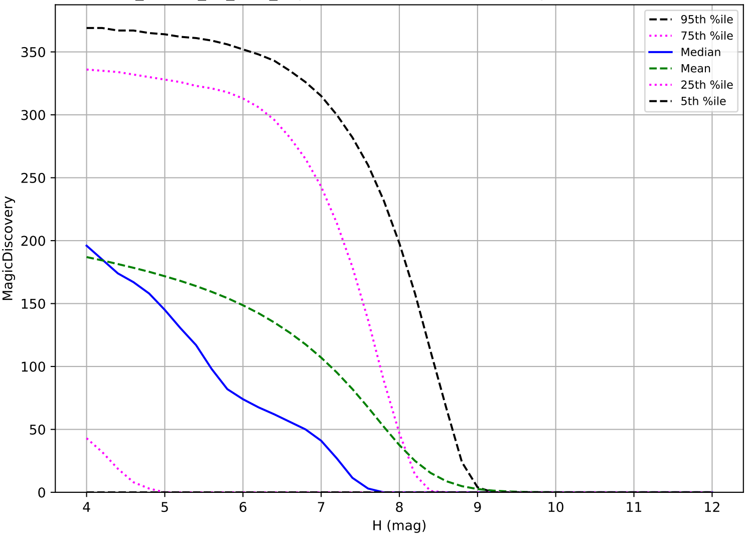
ddf_loaded_fl2_v3.4_10yrs: TNO 6 detections in 60 nights detection loss
