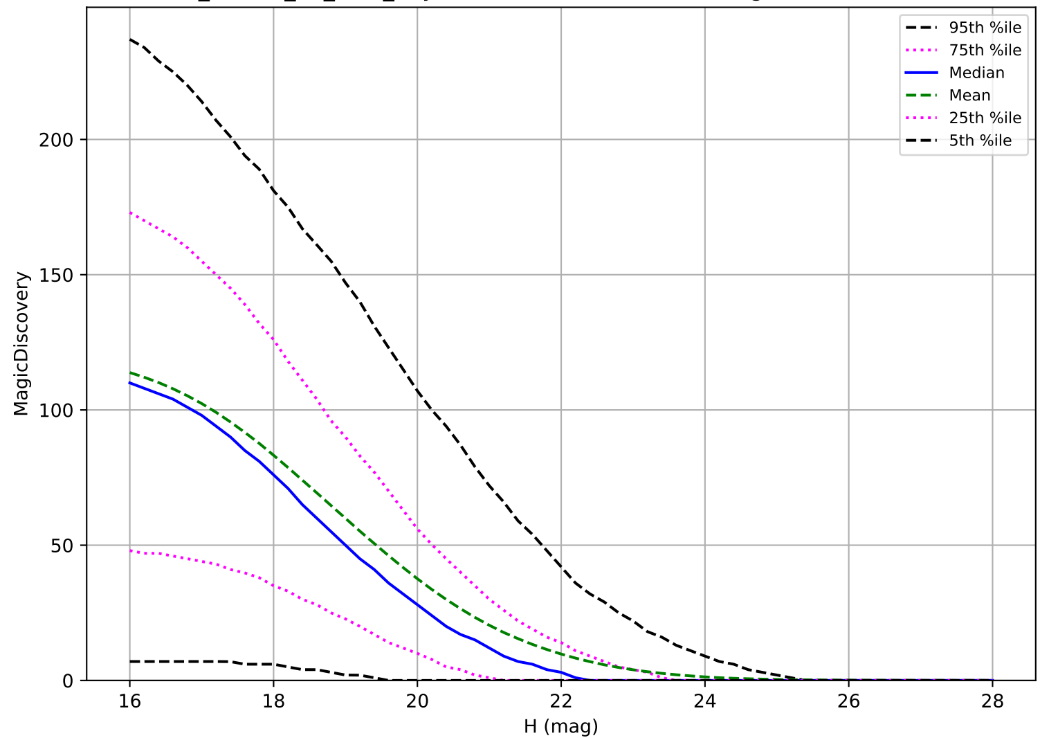
ddf_loaded_fl2_v3.4_10yrs: PHA 6 detections in 60 nights detection loss
