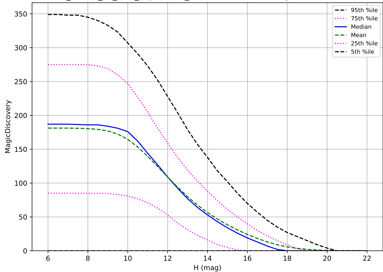
ddf_loaded_fl2_v3.4_10yrs: OCC_r5 6 detections in 60 nights detection loss
