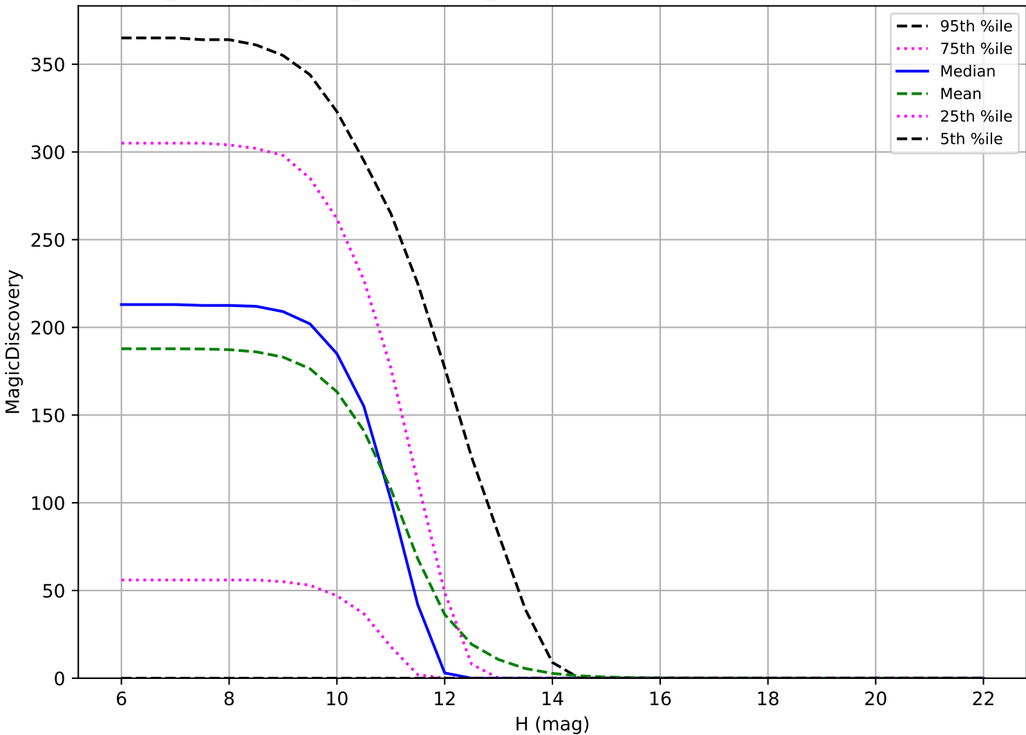
ddf_loaded_fl2_v3.4_10yrs: OCC_r20 6 detections in 60 nights detection loss
