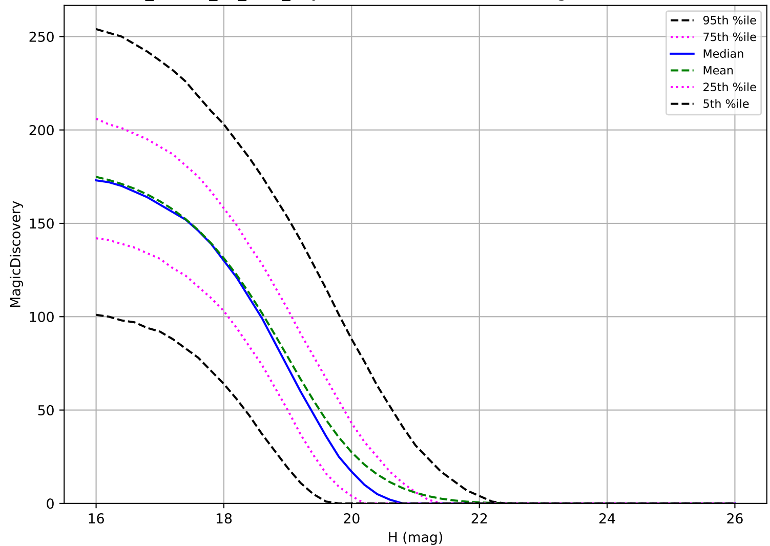
ddf_loaded_fl2_v3.4_10yrs: MBA 6 detections in 60 nights detection loss
