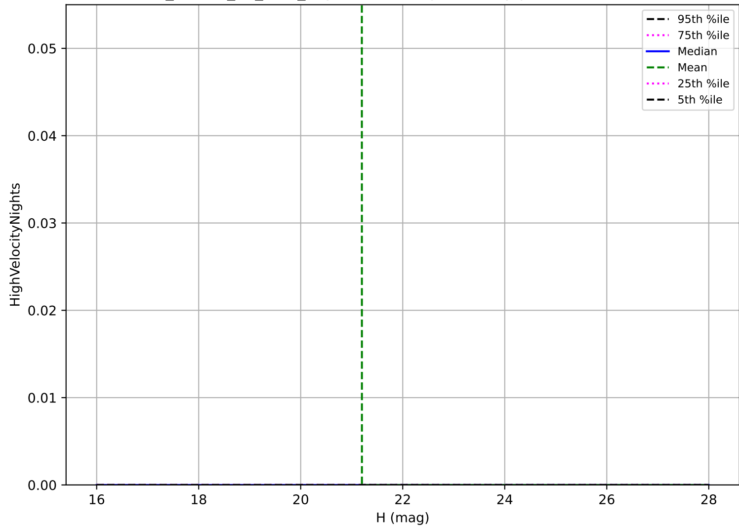
ddf_loaded_fl2_v3.4_10yrs: Vatira High velocity pair detection loss
