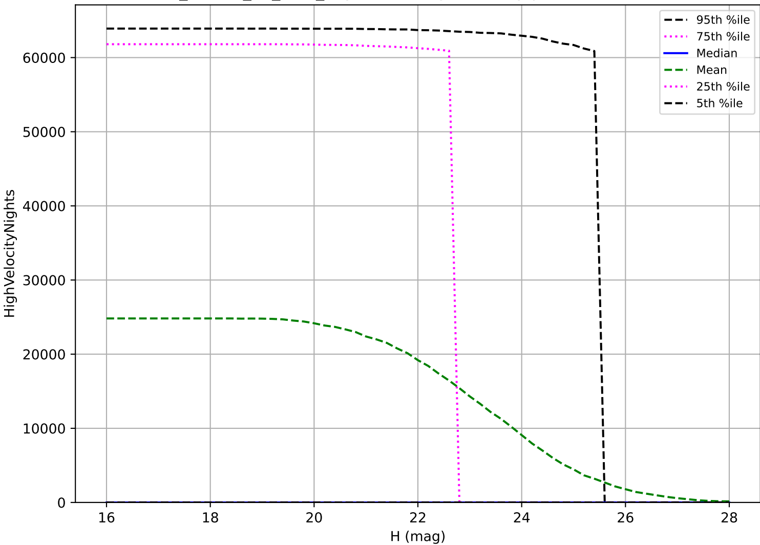
ddf_loaded_fl2_v3.4_10yrs: PHA High velocity pair detection loss
